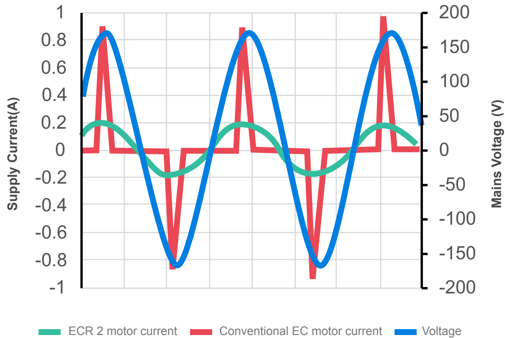
Figure 3: Current draw of an ECR motor vs. a typical EC motor
