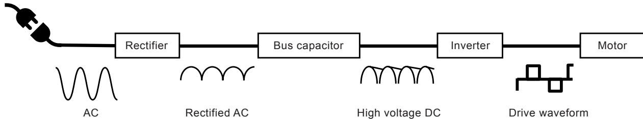
Figure 1: Typical EC motor block diagram
